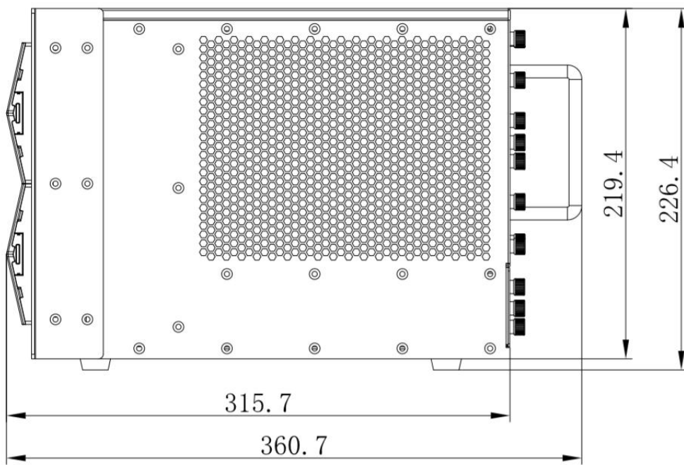
dimension drawing
