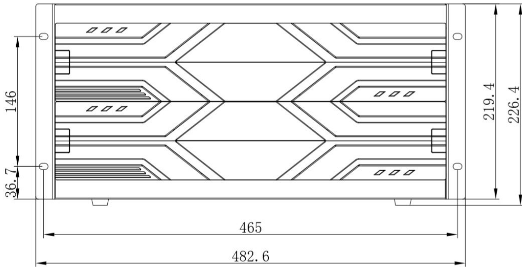
Front panel dimension drawing
