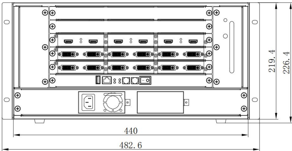
Rear panel dimension drawing
